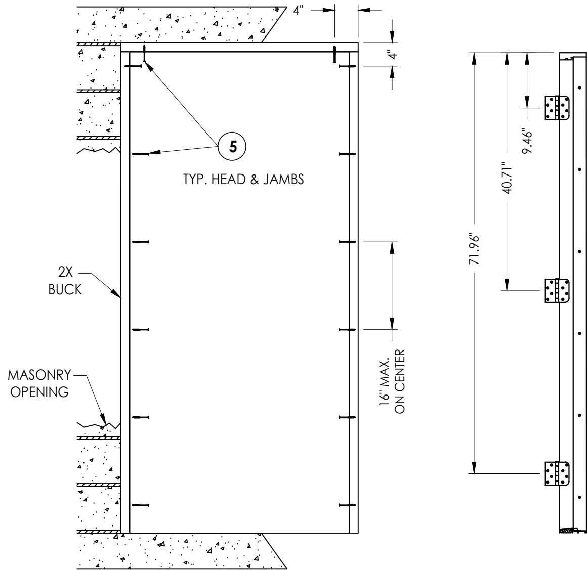
BUCK ANCHORING
