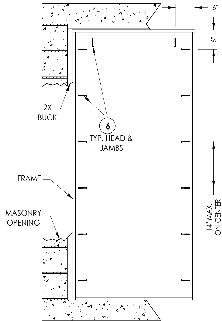
FRAME ANCHORING
